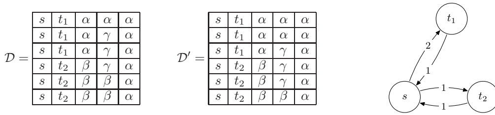
Figure 3: Two non-equivalent databases (left) giving the same database graph (right) for \mathcal{L} of Example 3.
