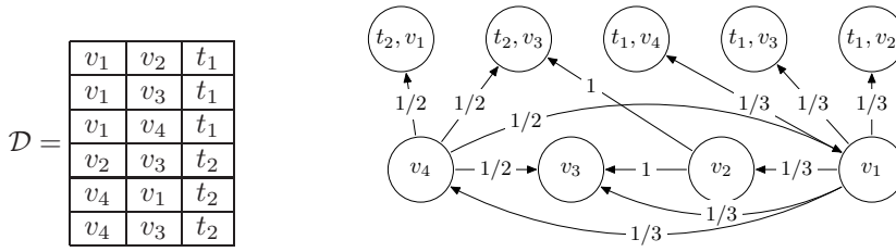
Figure 2: The database \mathcal{D} (left) and the database graph G_M of M = \langle \mathcal{D}, \mathcal{L}, f \rangle of Example 1 (right).
