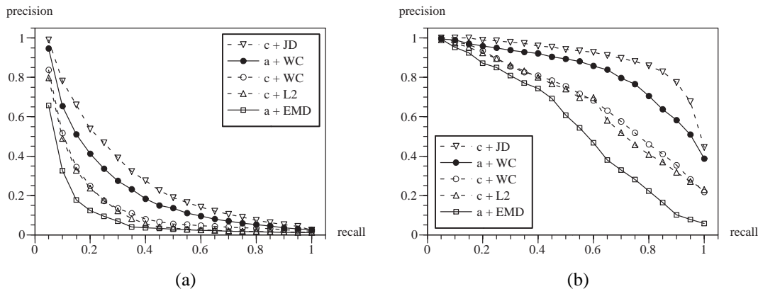
Figure 3. Precision-recall curves of various combinations of binning methods (c: clustered, dashed line; a: adaptive, solid line) and dissimilarities (JD: Jensen difference divergence, WC: weighted correlation, L2: Euclidean, EMD: Earth Mover’s Distance). (a) Scaling = 1/2, (b) scaling = 3/4.
