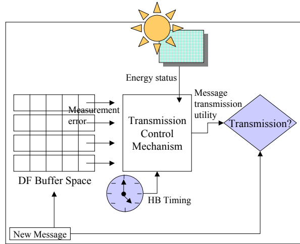
Fig. 3. Transmission Control Mechanism
