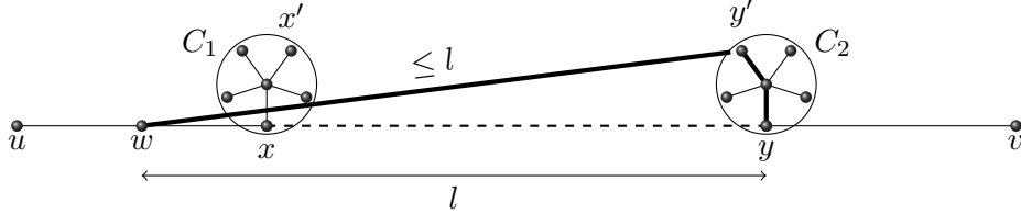
Figure 4.1: Path in H (thick) from w to y (via y' ) of length at most l + 2
