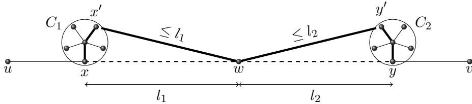
Figure 4.2: Path in H (thick) from x to y via x', w and y' of length at most l_1 + l_2 + 4
