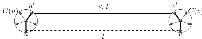
Figure 3.2: Path in H (thick) from u to v (via u' and v' ) of length at most l + 4
