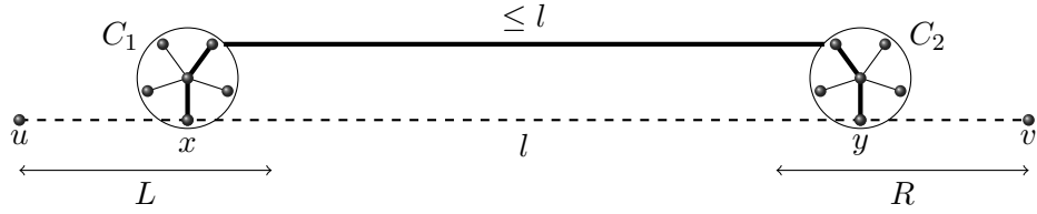
Figure 2.3: Path in H from C_1 to C_2 of length at most l
