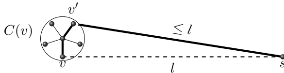
Figure 3.1: Path in H (thick) from s to v via v' of length at most l + 2
