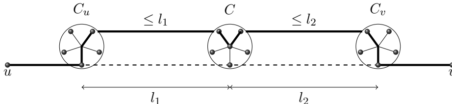
Figure 2.2: Path in H (thick) from u to v of additive stretch at most 6
