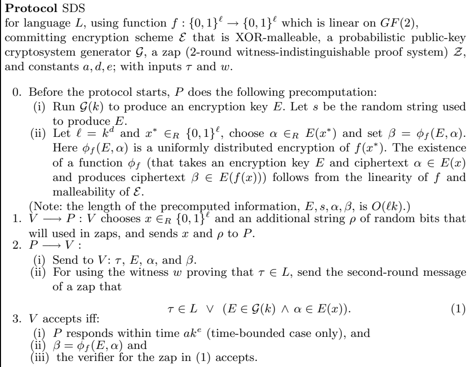
Fig. 1. Protocol SDS (simplification of Dwork-Stockmeyer [6] protocol).
