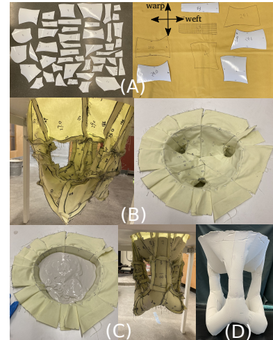
Figure 8: Fabrication pipeline. (A) Cut patches and orient them w.r.t to the warp/weft directions (B) stitched formwork suspended to a frame (C) formwork filled with liquid plaster (D) Demolded object after curing is complete
