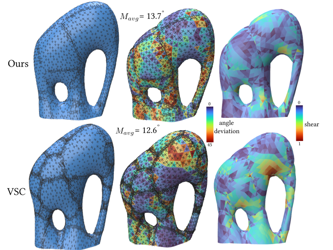
Figure 15: Strain directions comparison. Left: Strain field computed from the isotropic simulation. Middle: Strain field computed from the orthotropic simulation. Right: Normalized shearing computed from the right CG tensor \mathbf{C} (Eq. 3). M_{avg} shows the median deviation of the orthotropic strain field from the isotropic one. The isotropic simulation was run with the mesh produced by the respective segmentation methods (that remesh a lot along the seams) for ease of comparisons with the orthotropic strain field.
