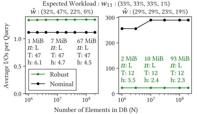
Figure 10: Impact of database size on performance. All tunings use the same expected workload w_{11} with executed workloads shown above each graph. Points at each power of 10 show m_{buf} and the tuning \Phi (L for leveling, T for tiering).
