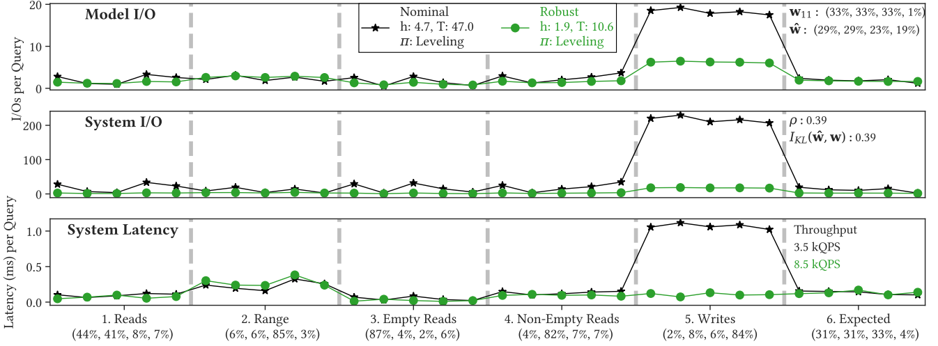
Figure 9: Sequence where \rho and I_{KL}(\hat{w}, w_{11}) closely match. Both system I/O and latency show reductions of up to 90%.
