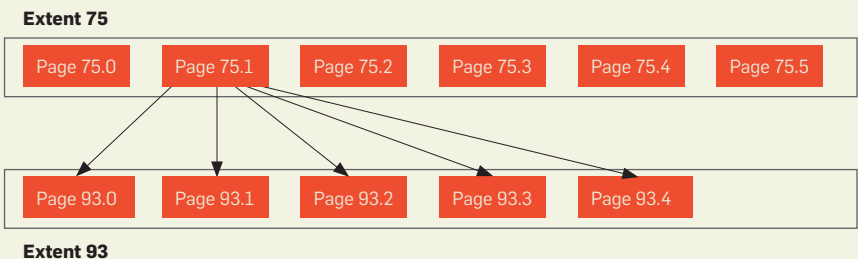
Figure 3: Pages and extents in an SB-tree.
