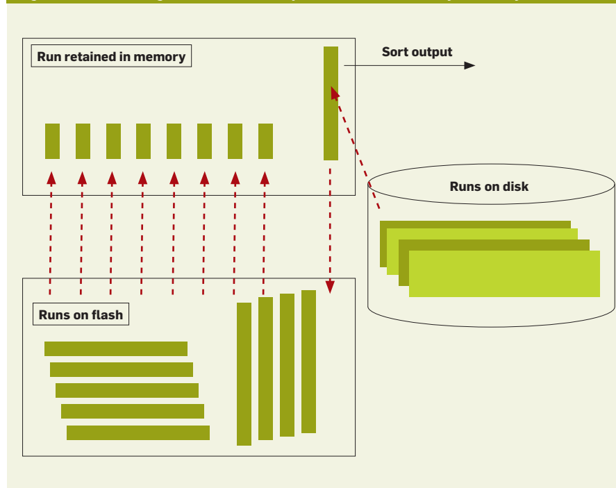
Figure 5: Graceful degradation with multiple levels in the memory hierarchy.
