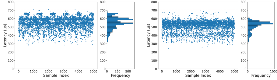
Fig. 9. Linux/TSN End-to-End Latencies with 62μs Window.
