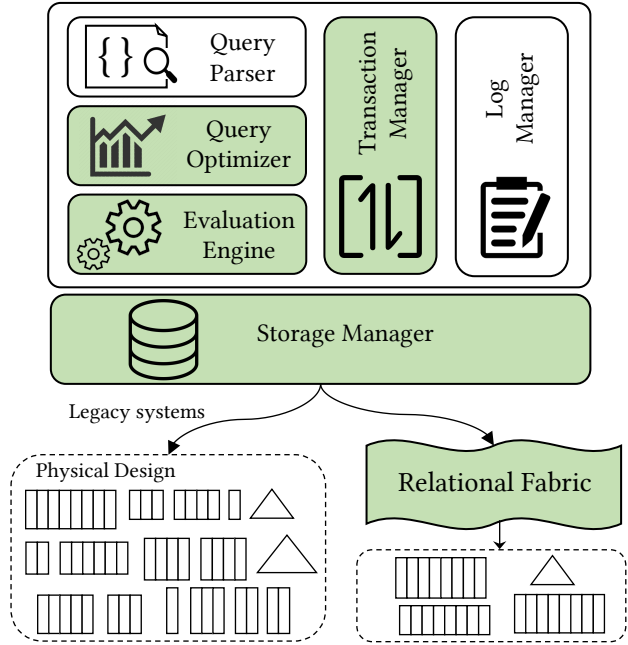
Fig. 4: Relational Fabric enables opportunities for innovation across the entire data system architecture. It simplifies physical design, provides more options for query processing and supports efficient multi-version concurrency control.
