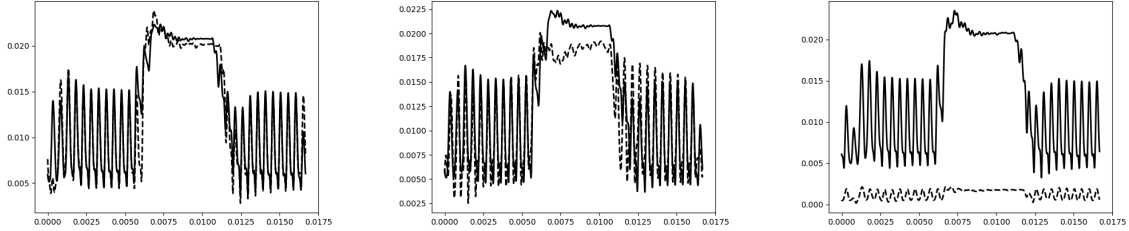
(a) Different signals of the same content of the same screen, taken using the close-range setup. (b) Signals of two different screens, taken using the standard setup. (c) Signals of different screens, one (solid) taken in close-range and one (dashed) taken from a distance using the parabolic dish.
