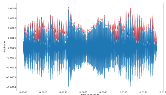
(d) Blue: The acoustic signal after applying a 27.5–38 kHz bandpass filter around the screen’s carrier. Red: amplitude demodulation of the blue signal. Notice the inverse correlation between the amplitude of the red signal and the brightness of pixel lines.
