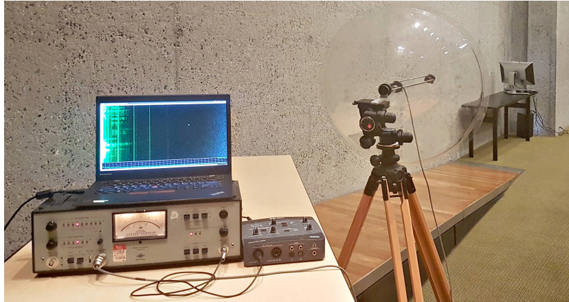
Figure 3.1: Extracting an image from a screen using a parabolic microphone at a distance of approximately 5 meters.
