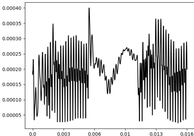
Figure 2.7: The output trace of the image of 2.5–a, using T = 0.9 , S = 3206 , d = 3 . This is visually indistinguishable from the product of chunking and averaging using the vsync probe (see Figure 2.6).
