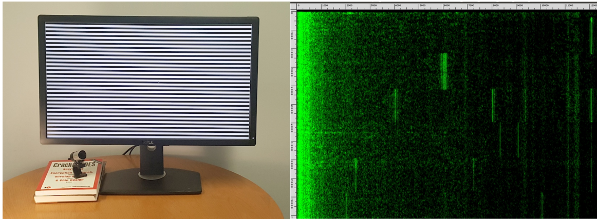
(a) Microsoft LifeCam Studio webcam positioned below a LED-backlit Dell U2713H screen, recorded through a Hangouts call. The frequency axis range is 0-13 kHz, due to the lower sampling rate used by Hangouts.
