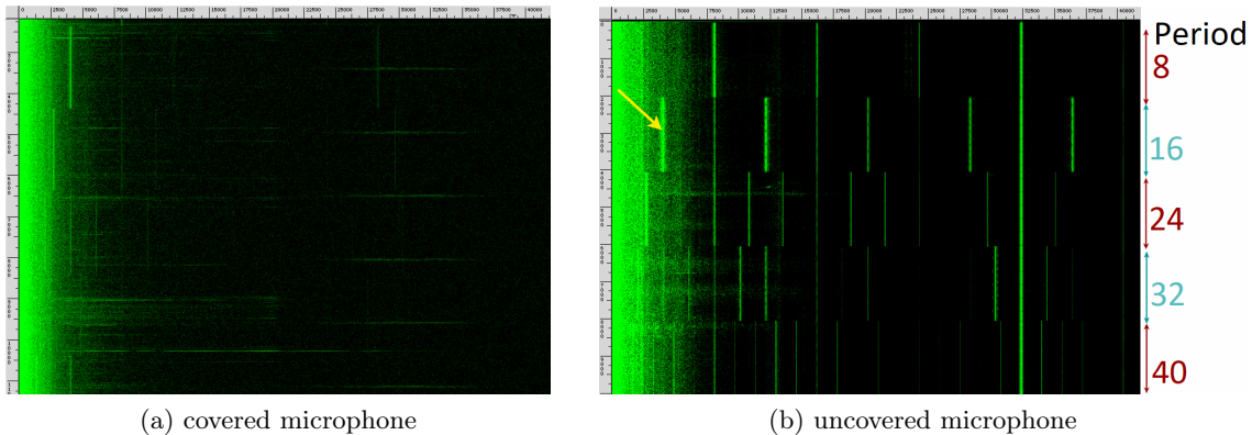
Figure 2.2: (right) Spectrogram of acoustic signals emitted by Soyo DYLM2086 screen while displaying alternating Zebra patterns. Notice the difference in the screen’s acoustic signature caused by the change in periods of the displayed Zebra pattern. (left) Spectrogram of a recording in an identical setting, but with the microphone covered by a thick piece of cloth. In both spectrograms, the horizontal axis is frequency (0-43 kHz), the vertical axis is time (10 sec), and intensity is proportional to instantaneous energy in that frequency band. The yellow arrow marks the 4 kHz leakage signal expected to be produced by a Zebra pattern with a period of 16 pixels.
