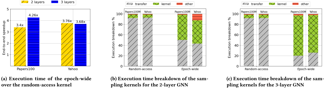
Figure 5: Preliminary evaluation results on two real-world graphs using GraphSAGE.
