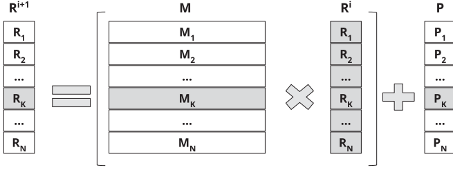
Fig. 9. PageRank computation as a vector-matrix multiplication. Vector R_i represents the computed ranks at iteration i , M is the input graph's adjacency matrix, with values scaled to account for the damping factor, and P contains the transition probabilities.
