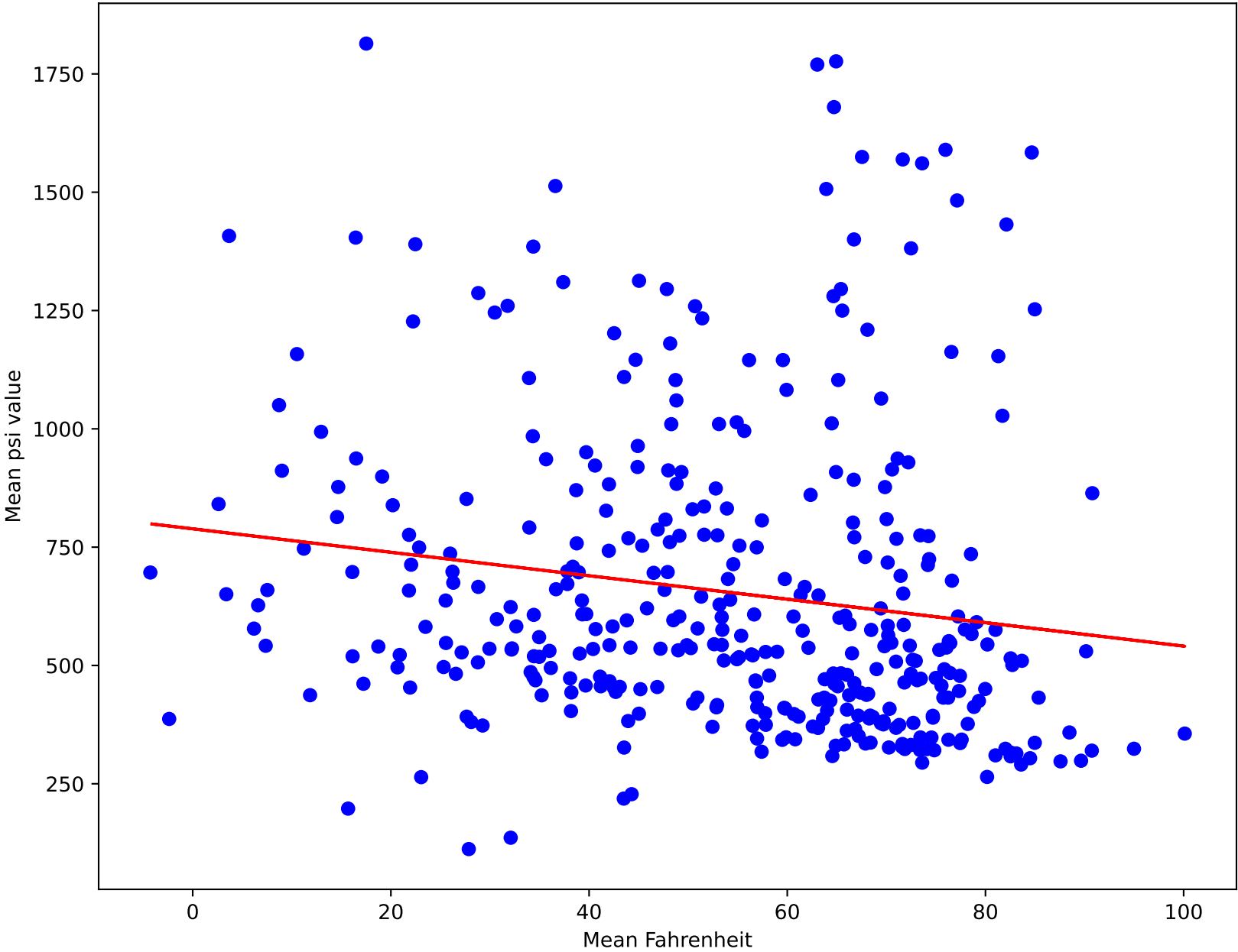
Device BU #43 West Loading Dock ( R^2=0.03 )
