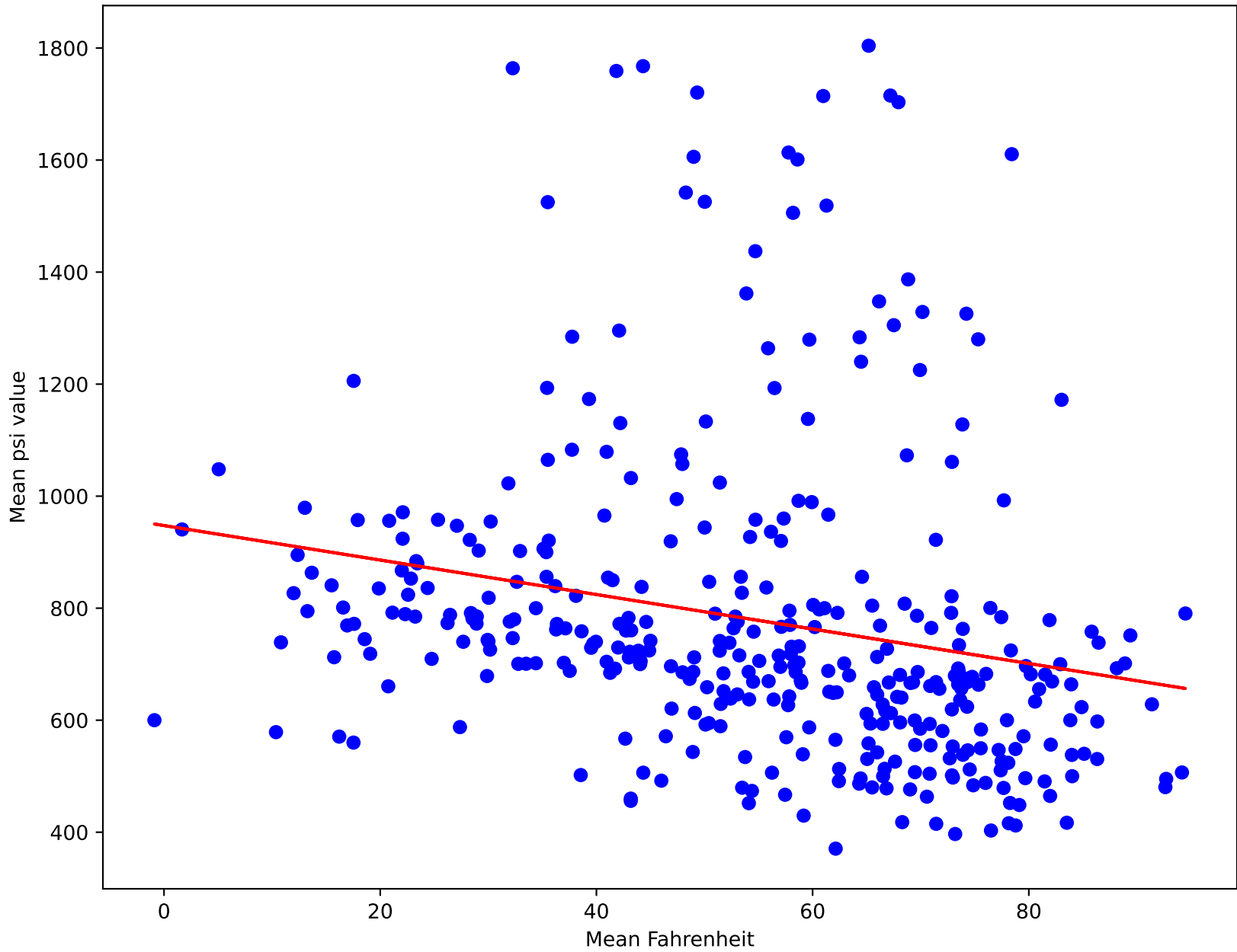
Device BU #72 Rafik B Hariri 20 YD ( R^2=0.05 )
