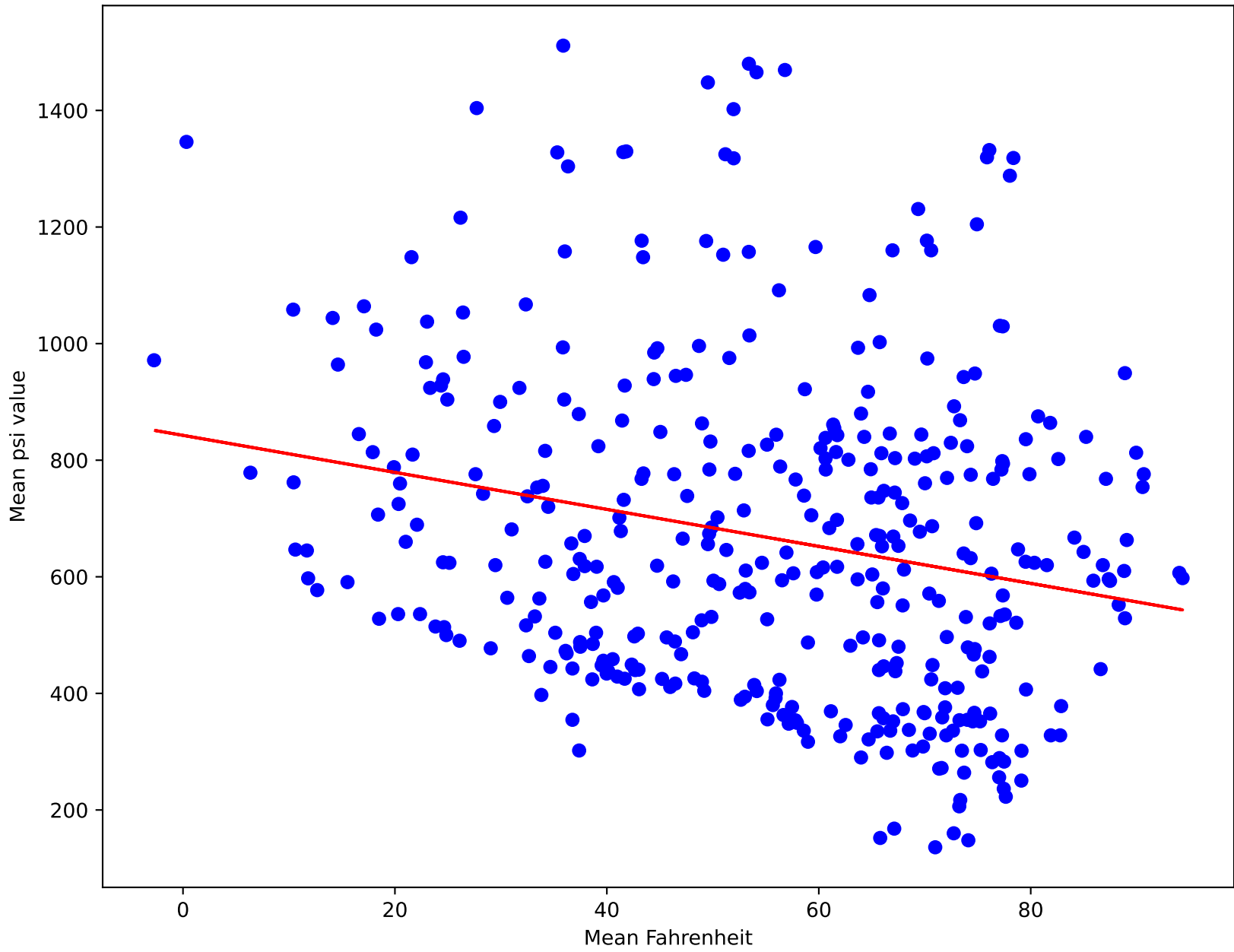
Device BU #90 - School of Law 35 ( R^2=0.05 )
