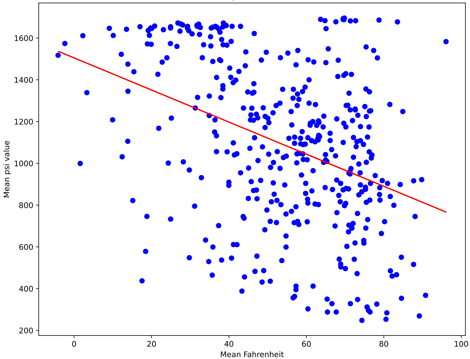
Device BU Fenway Trash 20 Yd ( R^2=0.15 )
