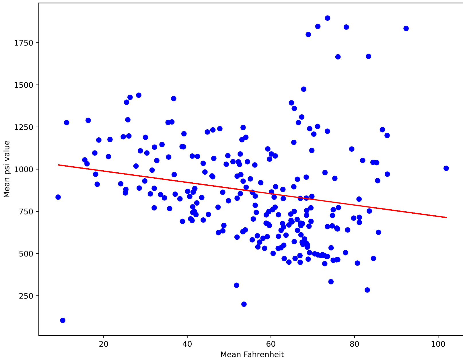
Device BU #102 Student Health Services 35 Yd (R 2 =0.04)
