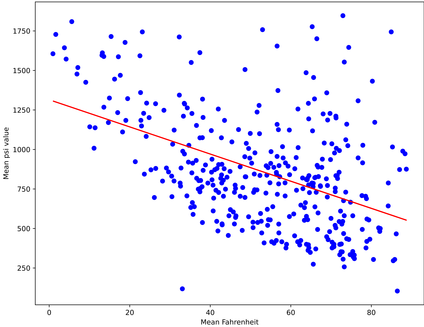
Device BU 685 Comm Ave ( R^2=0.22 )
