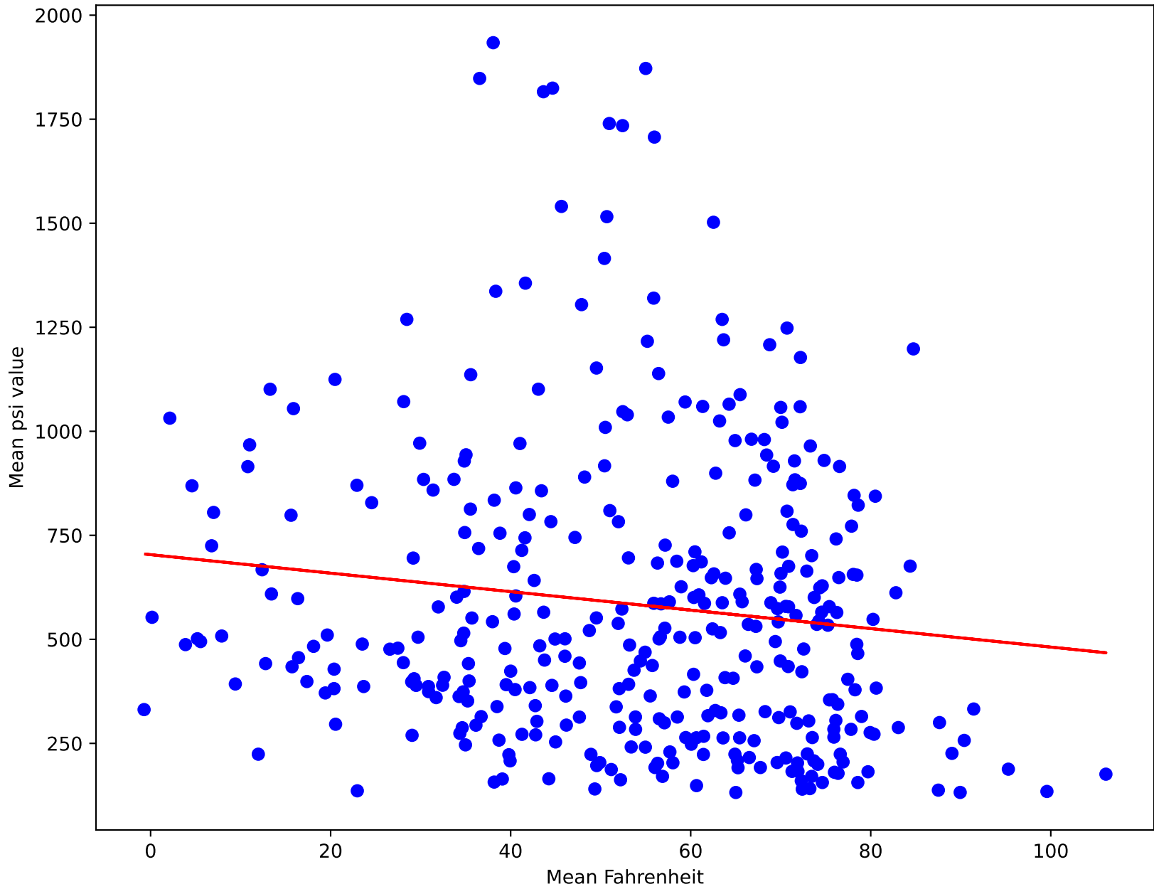
Device 140 Bay State ( R^2=0.02 )
