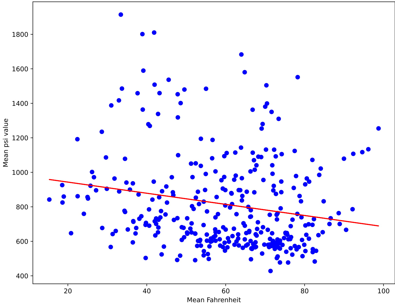
Device BU #93 George Sherman Union 35 Yd (R 2 =0.04)
