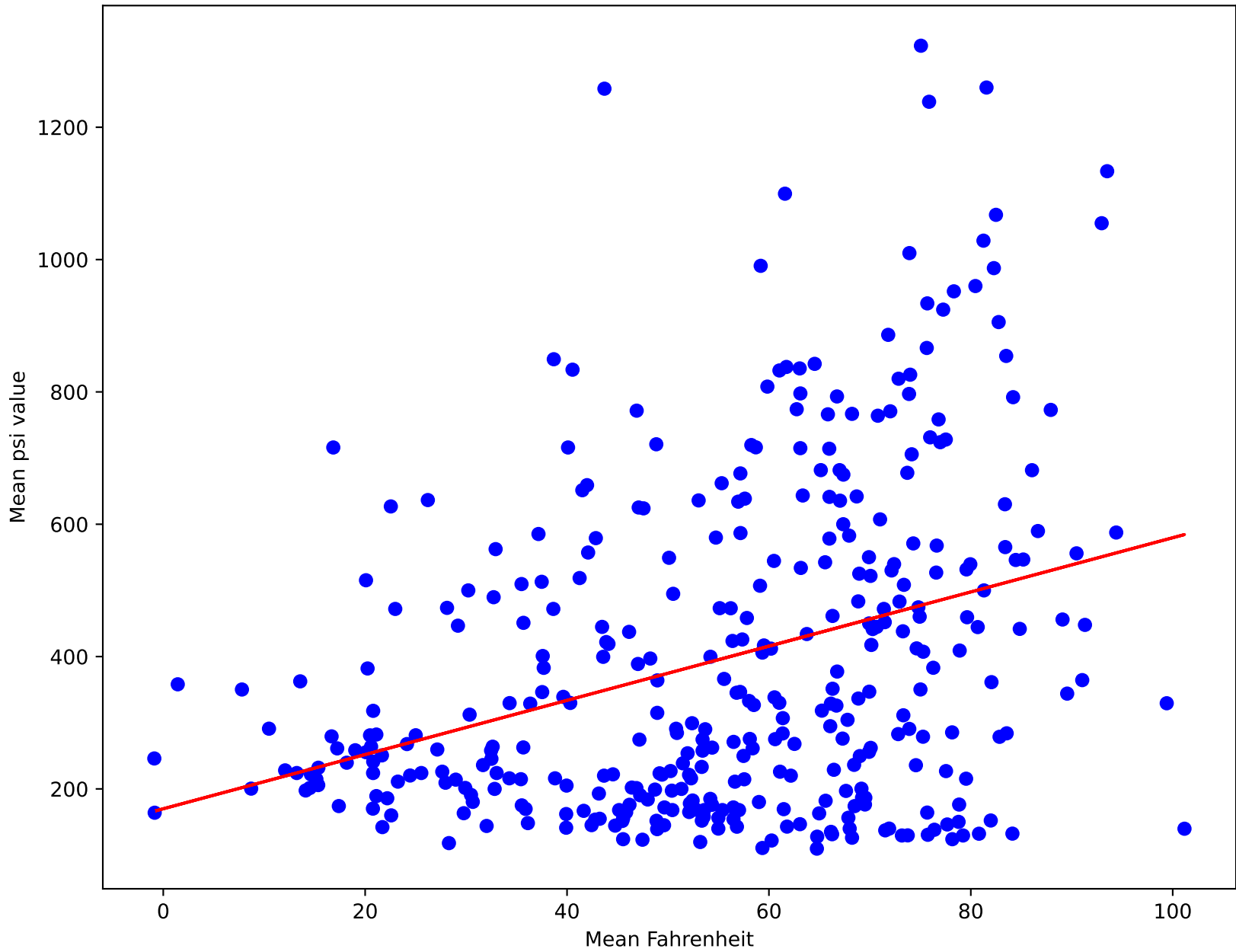
Device BU #38 Life Sciences 20 Yd ( R^2=0.11 )
