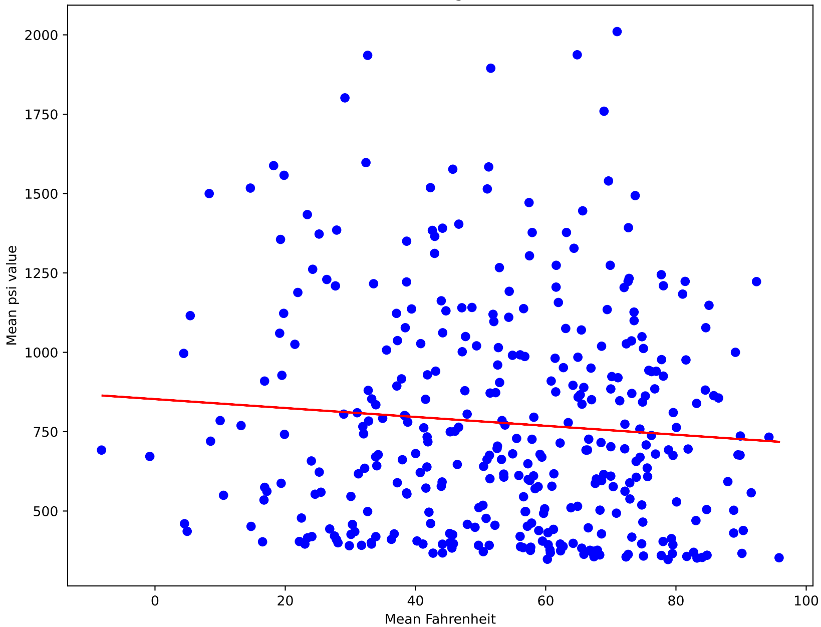
Device BU #48 Student Village #2 20 Yd ( R^2=0.01 )
