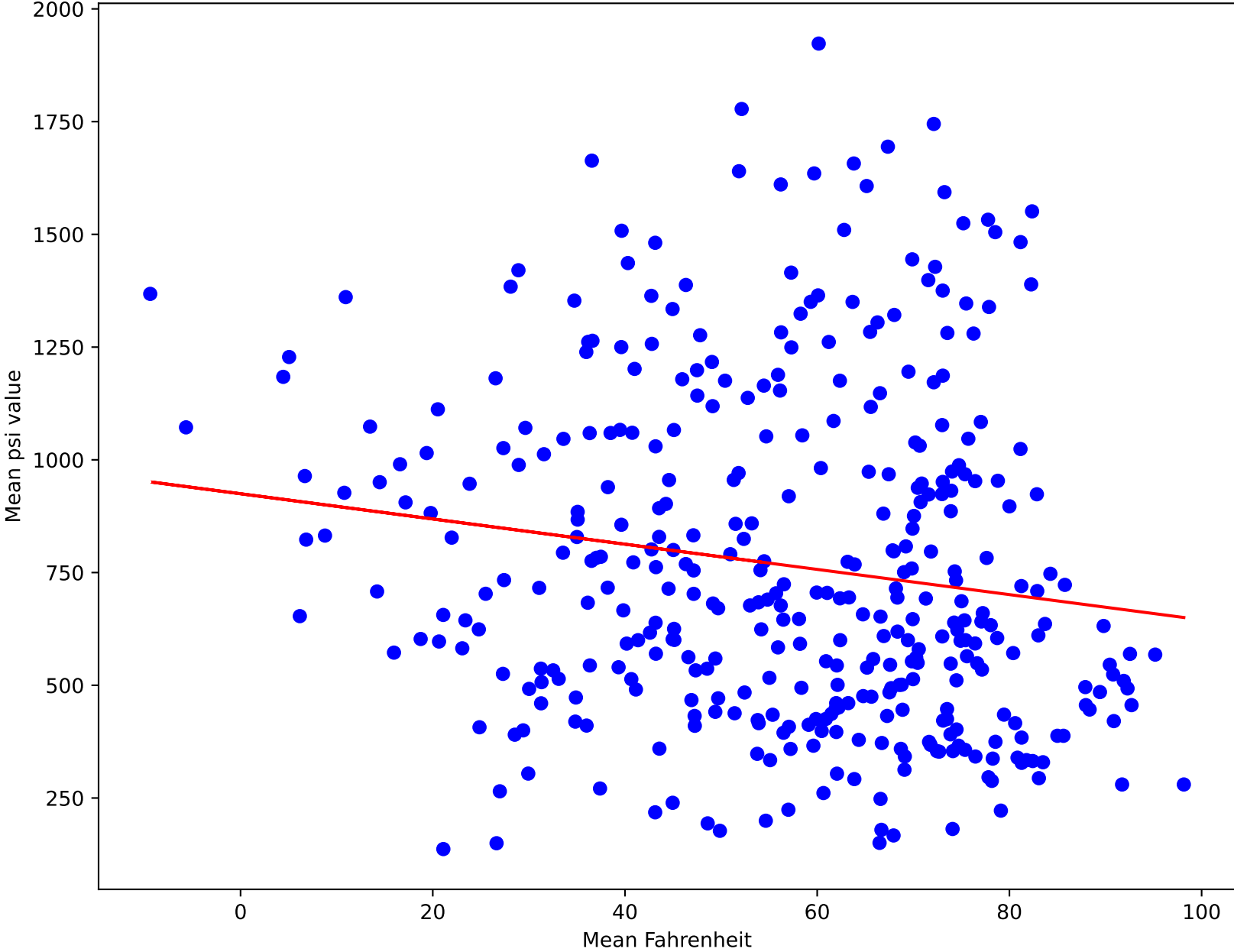
Device BU #46 30 Bay State 20 Yd ( R^2=0.02 )
