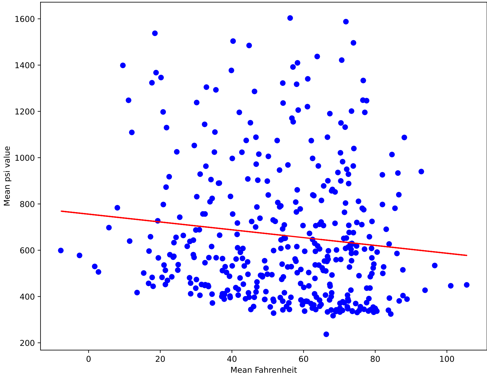
Device BU #2 Student Village 35 Yd (R^2=0.01)
