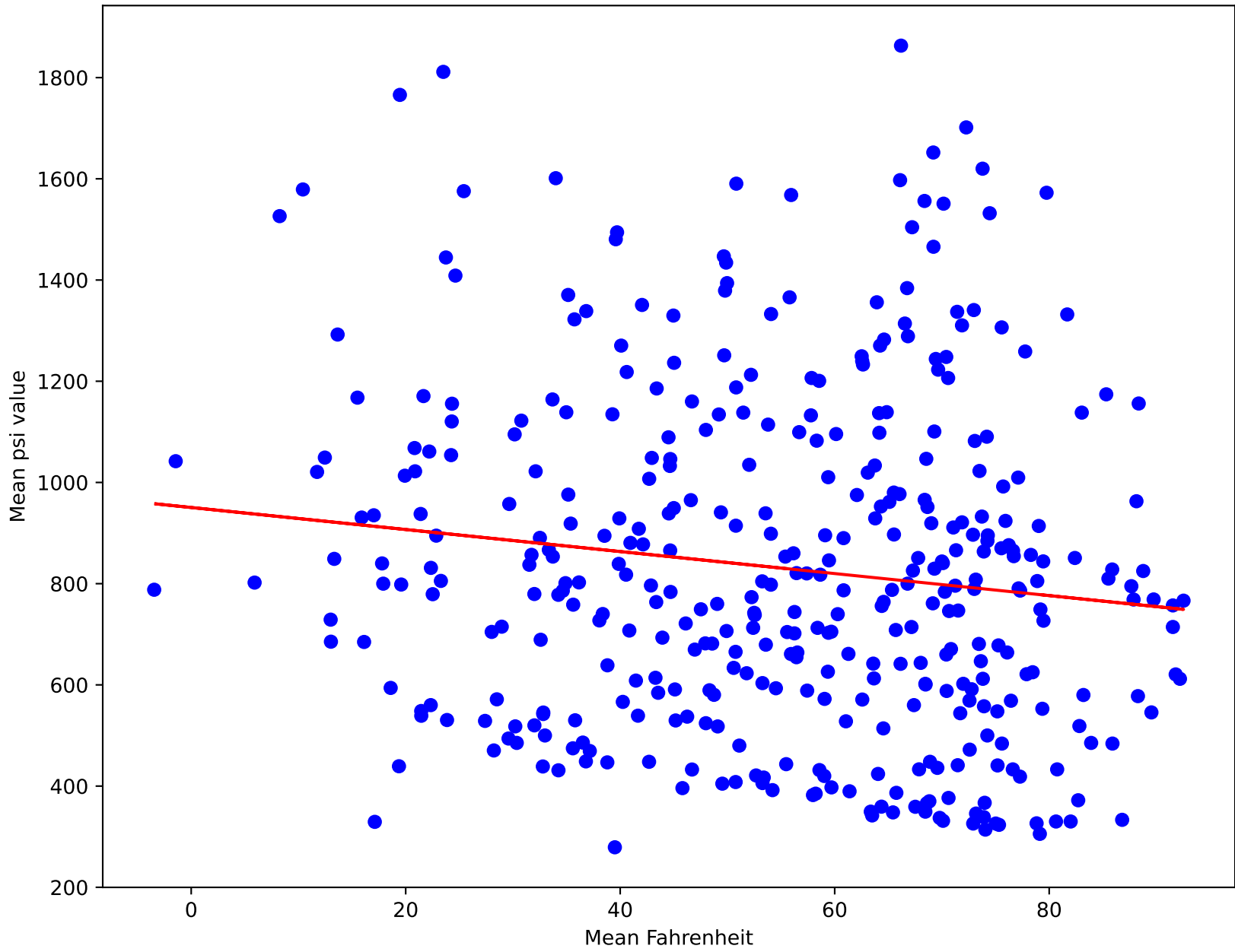
Device BU #18 - Warren Hall 20 Yd ( R^2=0.02 )
