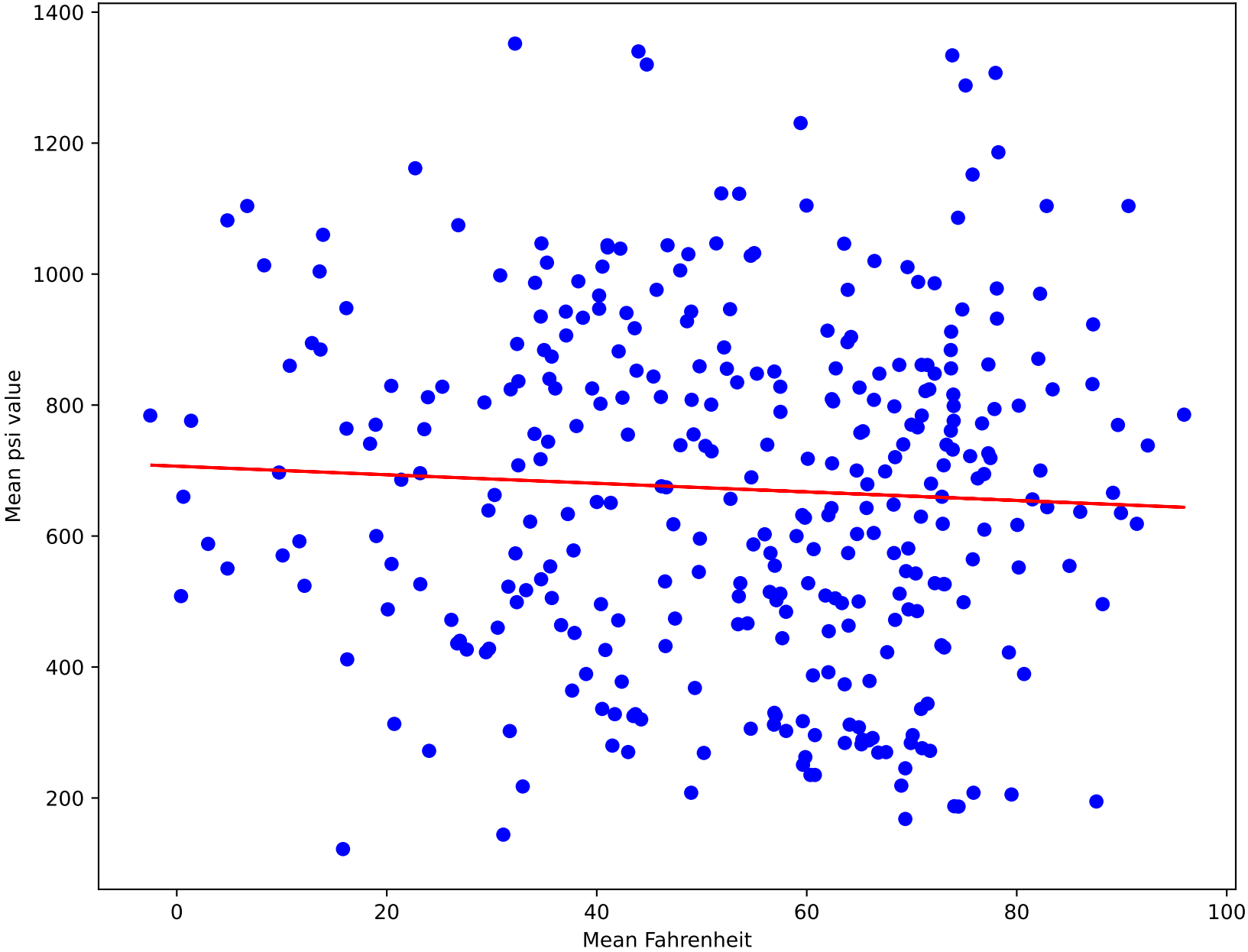
Device BU #96 808 Comm Ave 35 Yd ( R^2=0.00 )
