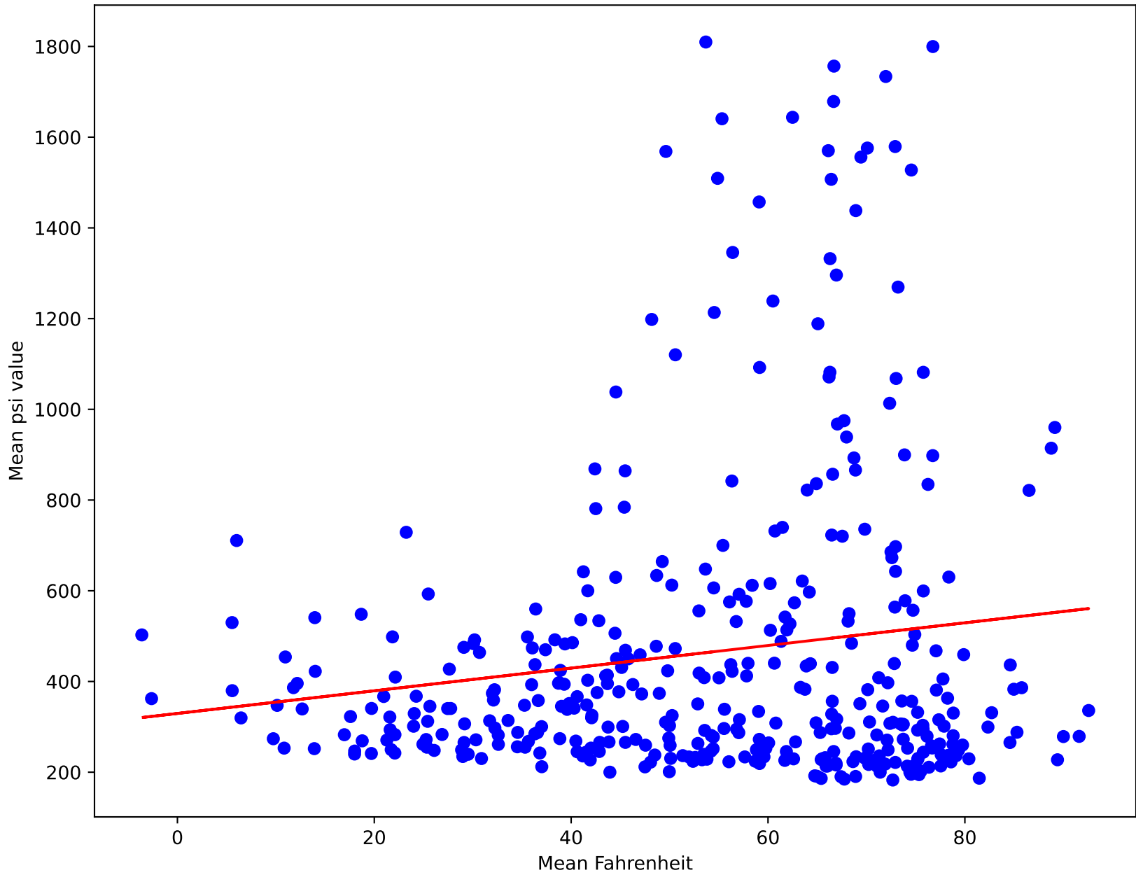
Device BU #82 Warren Towers 35 Yd ( R^2=0.02 )
