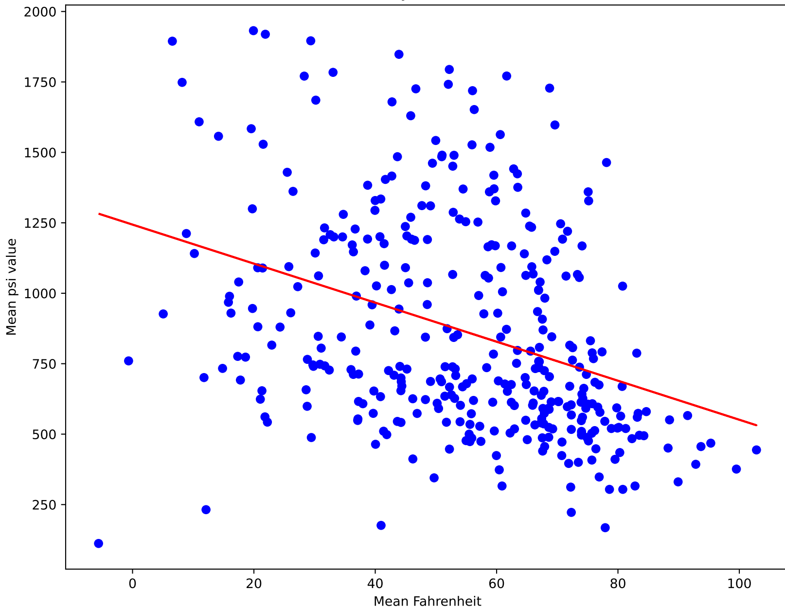
Device BU #4 Yawkey Center 15 Yd ( R^2=0.13 )
