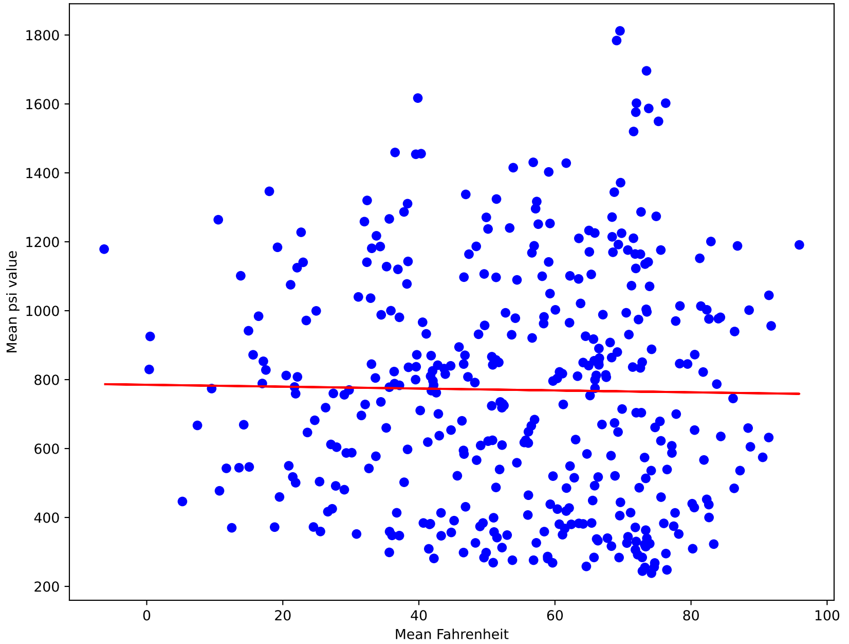
Device BU #35 22 Babbit 35 Yd ( R^2=0.00 )
